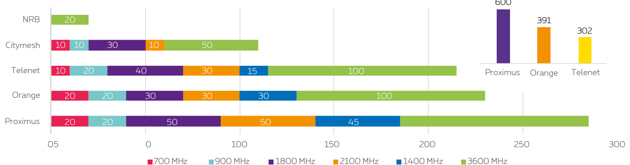
Spectrum holding per operator (MHz)
